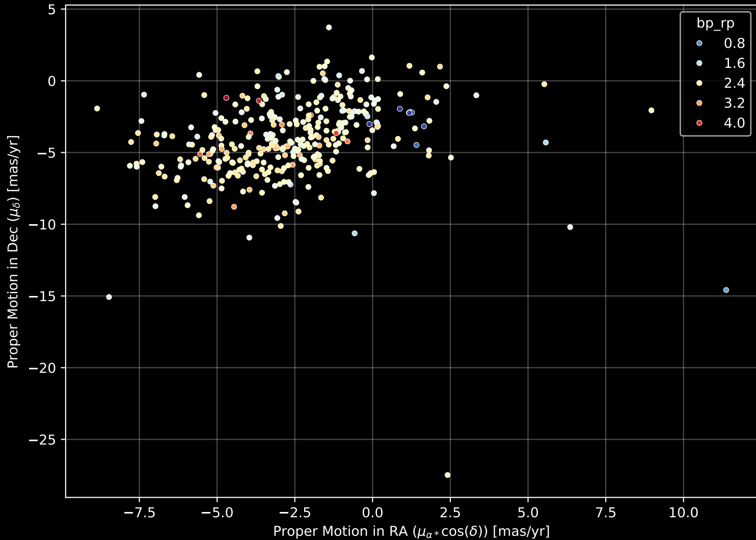
APOGEE DR17 Field: [350+04] Proper Motion Diagram (n= 343)
