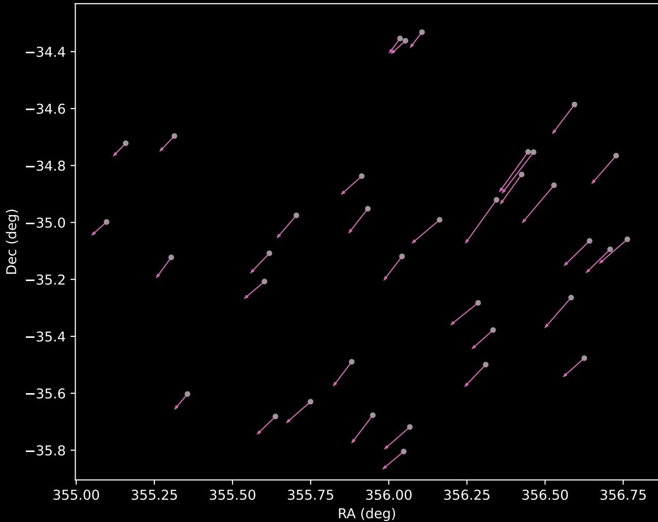
APOGEE DR17 Cluster 12 Proper Motion Vectors (n=36)
