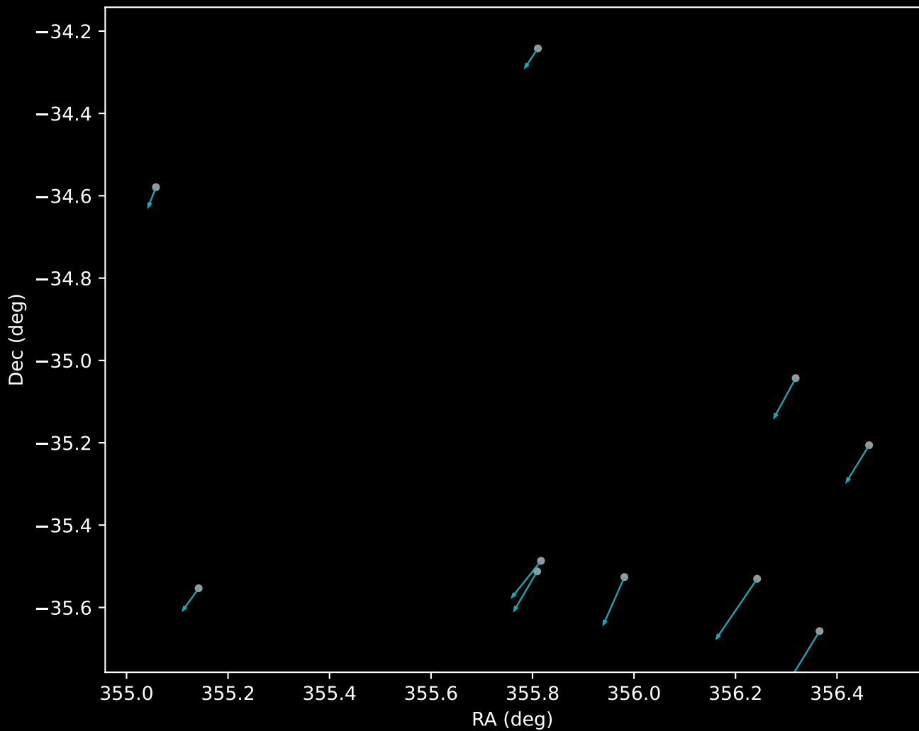
APOGEE DR17 Cluster 18 Proper Motion Vectors (n=10)
