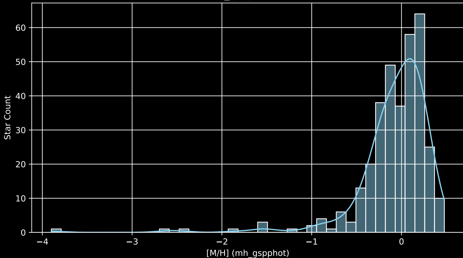
APOGEE DR17 Field: [350+04 [M/H] (mh_gspphot) (n= 338)
