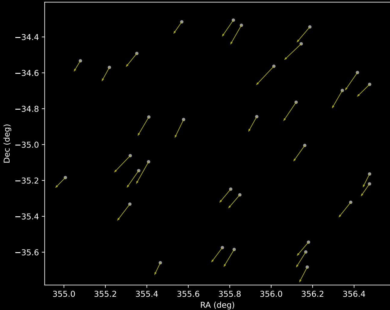
APOGEE DR17 Cluster 16 Proper Motion Vectors (n=33)
