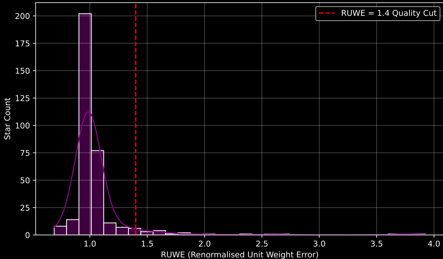
GAPOGEE DR17 Field [350+04] RUWE Distribution (n= 342)
