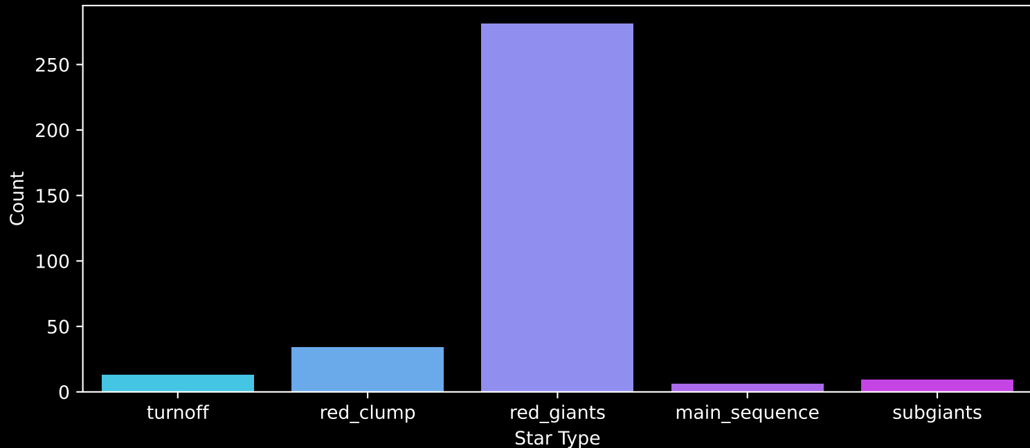
APOGEE DR17 Field: [350+04] Count plot of Star Type
