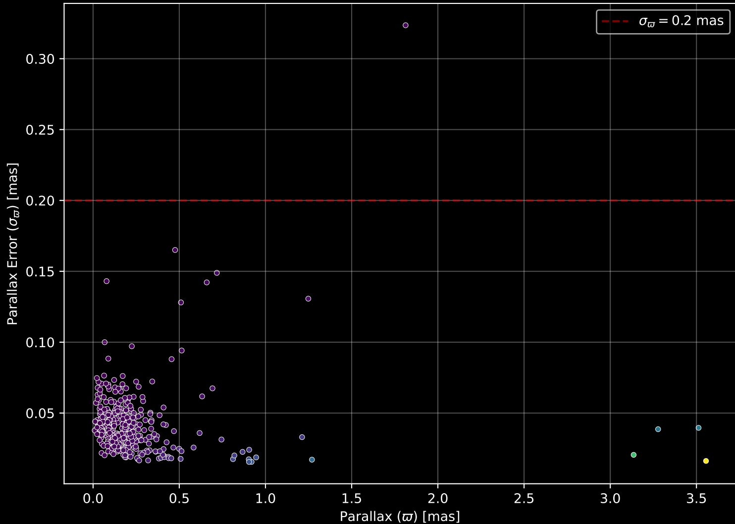
APOGEE DR17 Field: [350+04] Parallax Quality (n= 343)
